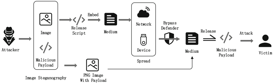
Fig. 1. System and threat model.
