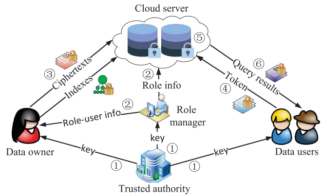
Fig. 2. System model of REKS.
