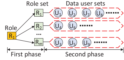
Fig. 4. Relationship between roles and users.
